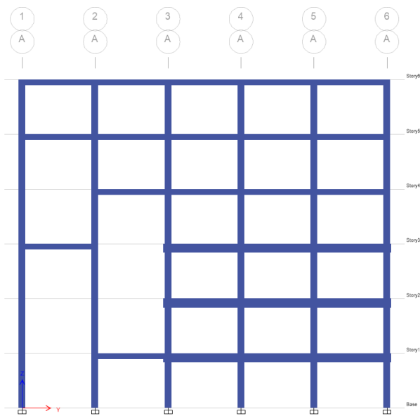
East elevation.
